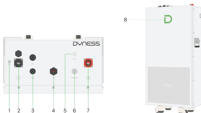
Figure 2-1 PowerBrick PLUS the Sketch of Front Interface
