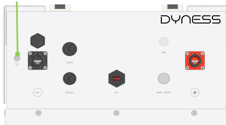
Figure 3-4 Location of grounding point
